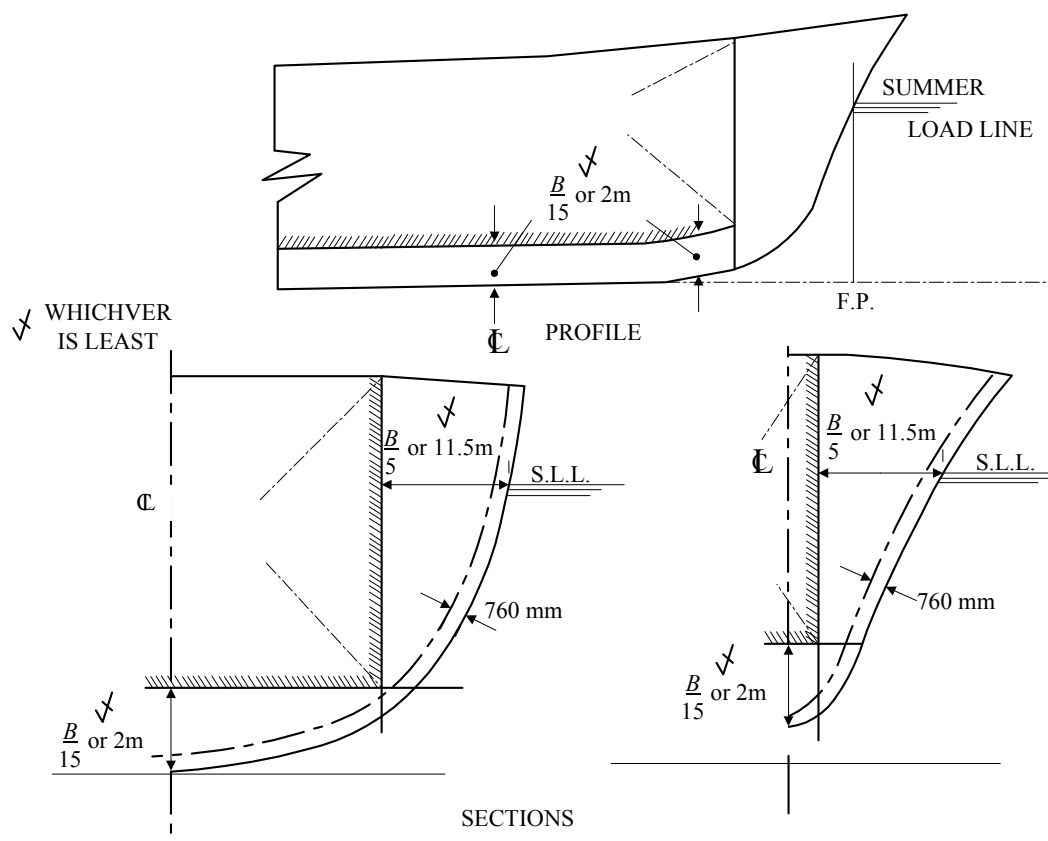
FIGURE 1 Tank location requirements as set out in 5C-8-2/6
