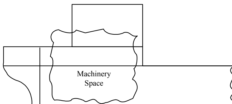
FIGURE 2 Longitudinal extent of damage to superstructure (5C-8-2/7.8 and 5C-8-2/8.1)
